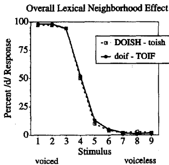
Figure 8. Group identification functions for the doish-toish and doif-toif series.
