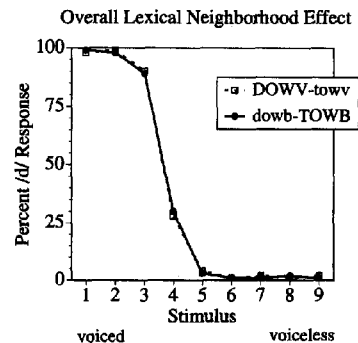
Figure 5. Group identification functions for the dowv-tovv and dowb-towb series.
