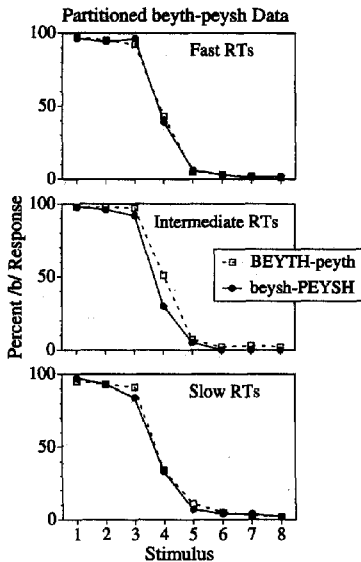
Figure 4. Group identification functions for the beyth-peysh and beysh-peysh series in three reaction time (RT) partitions: fast, intermediate, and slow.
