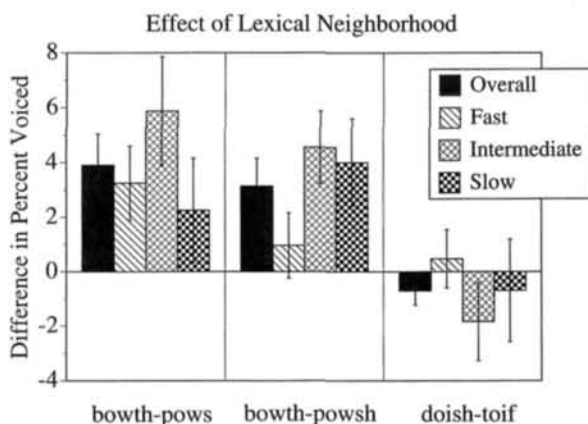
Figure 10. Neighborhood frequency effect on percentage of voiced responses for bowth-powv , bowth-powsh , and doish-toif series in both the overall data and each of the three reaction time partitions.
